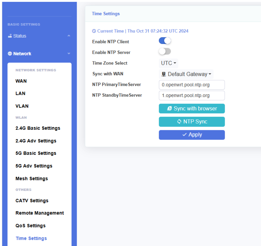
Figure 3-3-34: Time Settings
