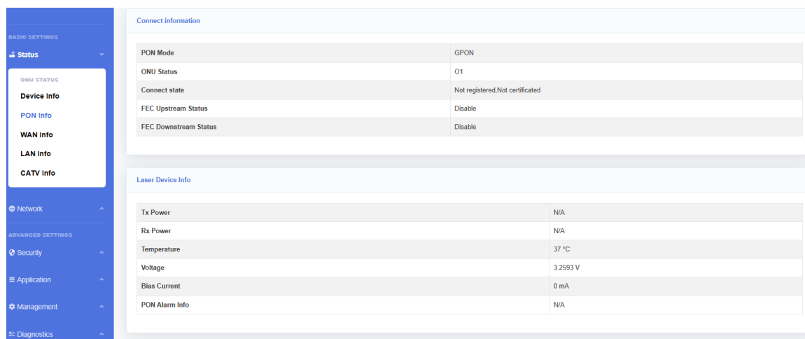
Figure 3-2-2: PON Info
