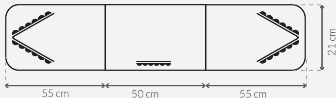
TOTAL LENGTH OF LIGHTBAR 160cm
