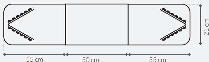
TOTAL LENGTH OF LIGHTBAR 160cm
