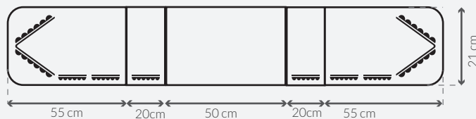
TOTAL LENGTH OF LIGHTBAR 200cm
