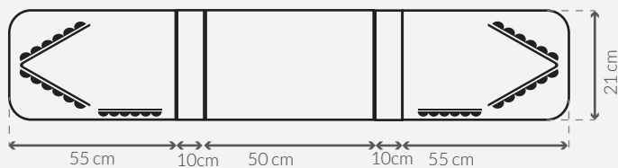
TOTAL LENGTH OF LIGHTBAR 180cm
