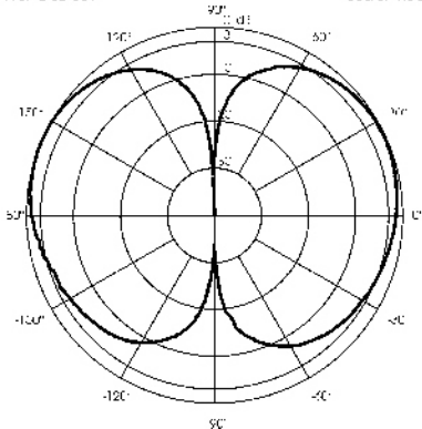
TYPICAL RADIATION PATTERN in E-plane at 145 MHz File: F 02 C31 Scale: none
