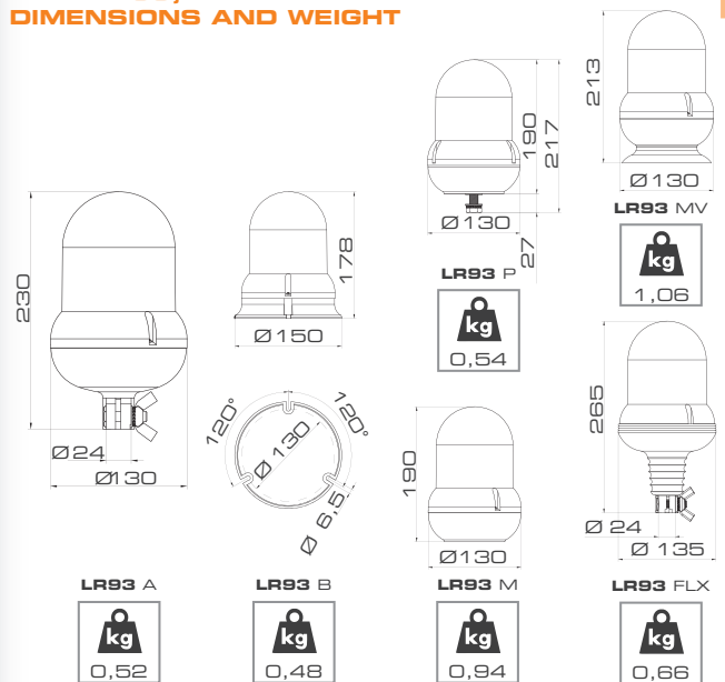
LR93 M ISO D BASE (MAGNETIC BASE, HELIX CABLE AND CIGARETTE LIGHTER PLUG)
