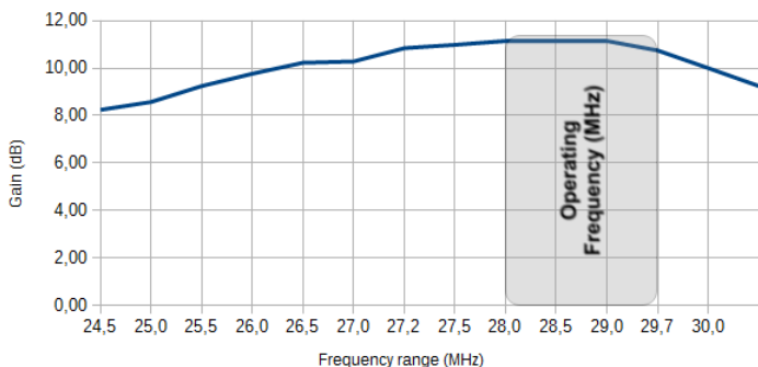
KL200 power Amplifier- Frequency Vs. Gain
