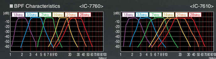
Showing primary BPF for HF amateur bands
