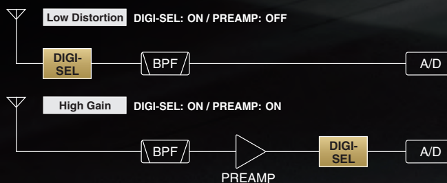
■ Block Diagram Overview
