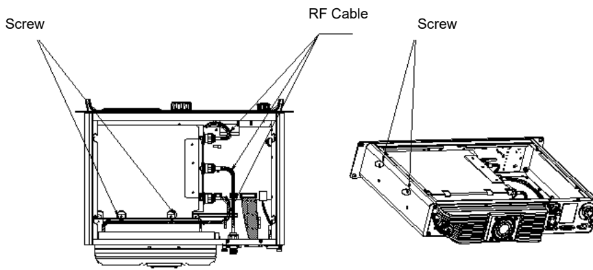
Duplexer with Front Side Facing Downwards
