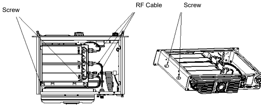
Duplexer with Front Side Facing Upwards
