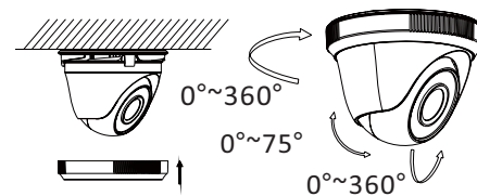
Figure 2-7 3-axis Adjustment
