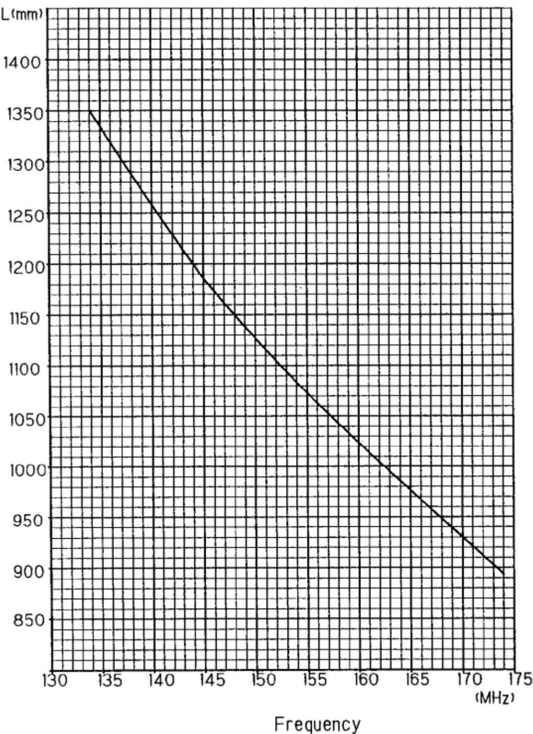
CUTTING CHART
